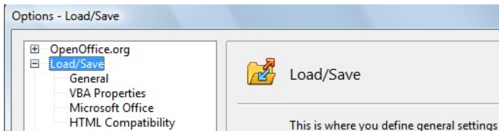
Figure 15: Load/Save options
